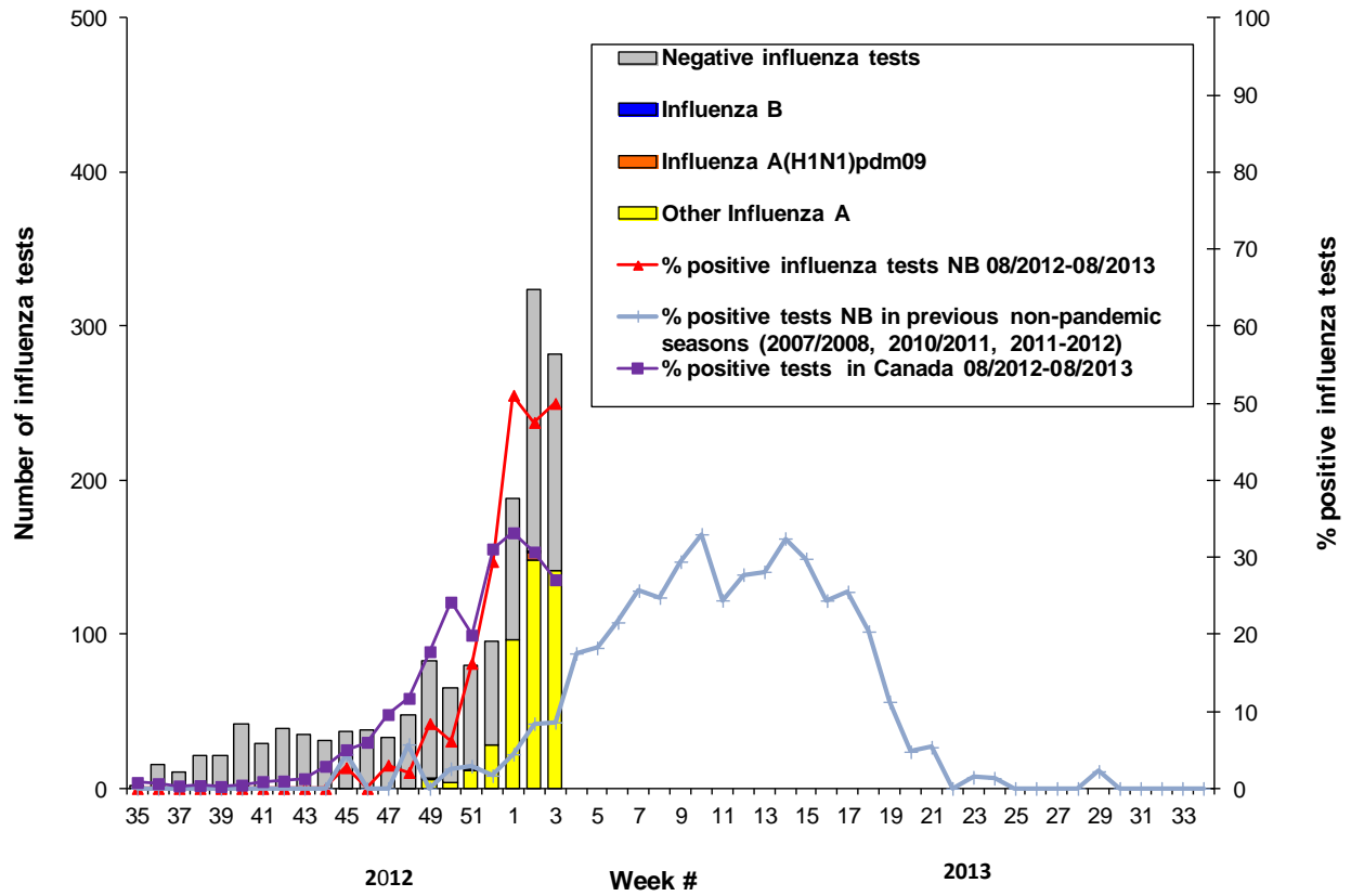
Graph 1: Number and percent of positive influenza specimens in New Brunswick, by week, up to January 19, 2013 (data source: G. Dumont lab results)
